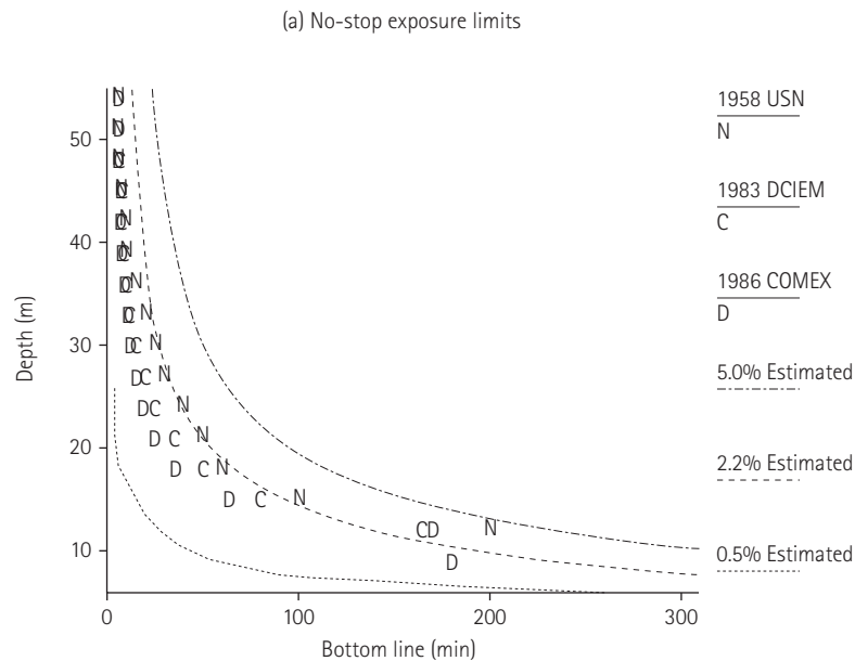
Fig. 10.2.4 No-decompression limits for three well established tables. Actual limits shown as points. Also shown are theoretical iso-risk curves representing 0.5, 2.2, and 5%
