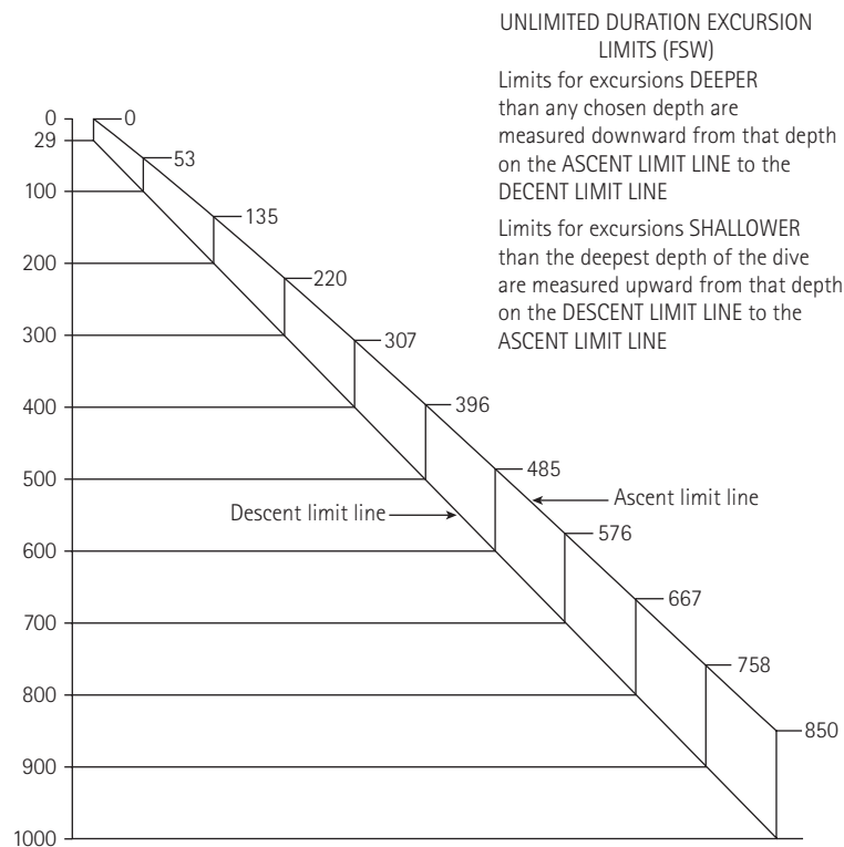
Fig. 10.2.5 USN unlimited duration helium–oxygen saturation excursion limits. Upward excursion limits in 100 ft
