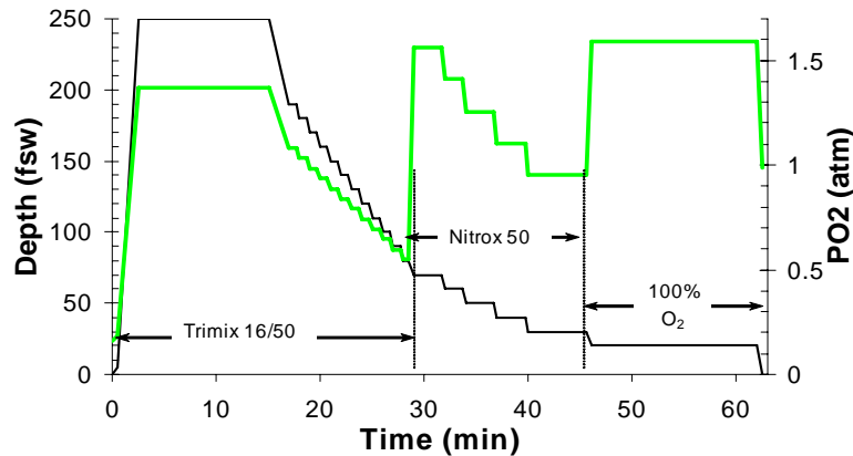
Figure 9. Dive profile for DCS Case 1 treated at Catalina Island (13).
