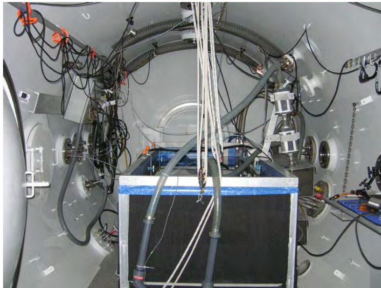
Figure 7. Water-filled ark inside a pressure chamber for immersing underwater breathing apparatus (UBA) during equipment tests.
