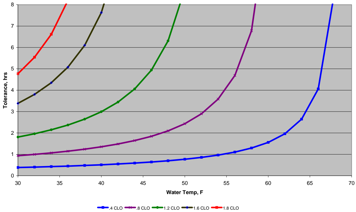
Figure 1. Estimated thermal tolerance limits for a resting diver (117 watts) in cold water with various suit insulation values.
