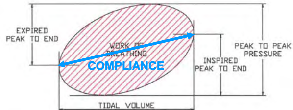
Figure 3b. Re-breathing equipment WOB, respiratory pressures and compliance.
