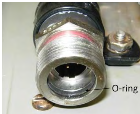
Figure 20. A damaged O-ring in this connector contributed to a fatality.
