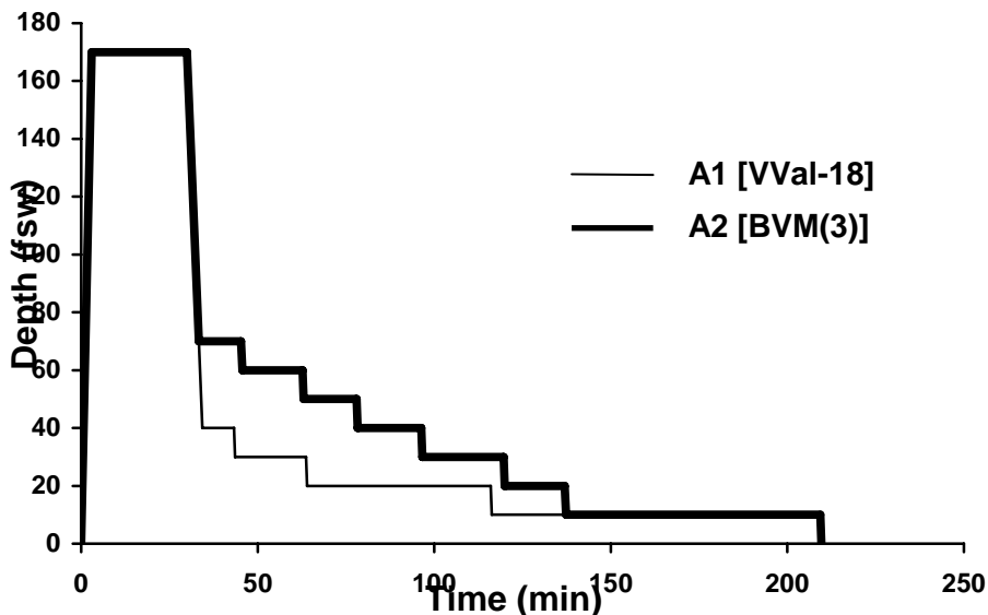
Figure 14. Overlay of the two 170 fsw/30 min air dive profiles man-tested at NEDU.
