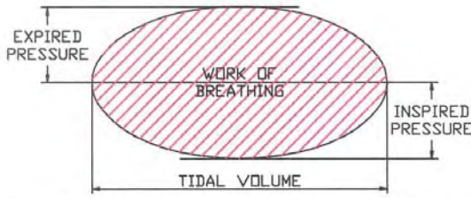
Figure 3a. Open-circuit equipment WOB and respiratory pressures.
