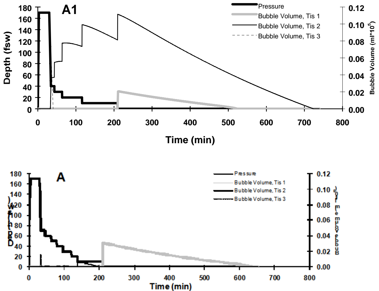
Figure 13. Hypothetical bubble-dependent DCS risk in two 170 fsw (52 msw)/ 30-min air dives identical except for the depth/time distributions of a 174-min total decompression stop time. Under the BVM(3) model, bubble formation in the A1 schedule causes the profile to incur an estimated DCS risk of 6.2%. Under the same model, the reduced extent of bubble formation afforded by the deep skew of decompression stop time in the A2 schedule causes the profile to incur an estimated DCS risk of 3.7%.
