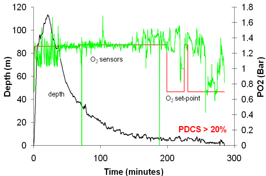
Figure 18. 200/ Britannic expedition dive profile (5-/-).
