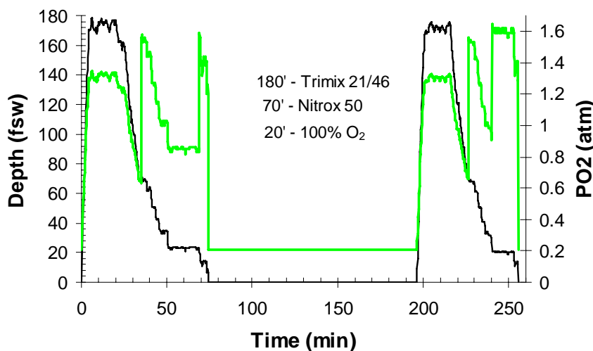
Figure 11. Dive profile for DCS Case 3 treated at Catalina Island (13).
