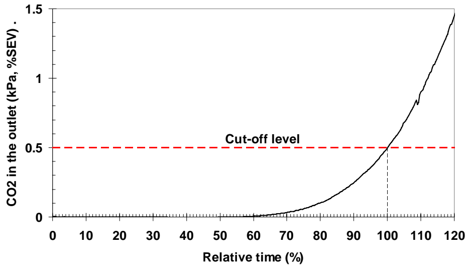
Figure 6. Commonly seen trace of the \text{PCO}_2 during an endurance run of a \text{CO}_2 scrubber.
