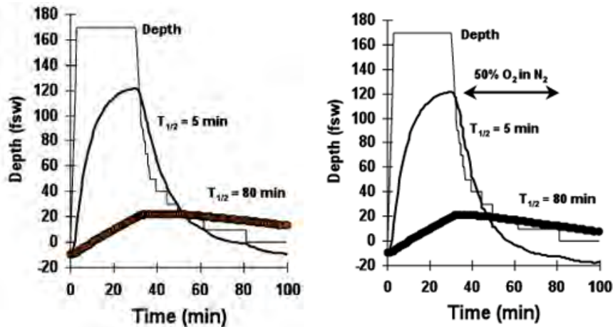
Figure 11. Depth and compartmental total dissolved gas tension profiles for a 170 fsw/30 min air dive with 1-min inserted deep stops at 10 fsw intervals starting at 90 fsw (left panel), and for the same dive with a breathing gas switch to higher FO_2 at the first of the inserted stops (right panel). The gas switch causes more rapid gas elimination in all compartments.
